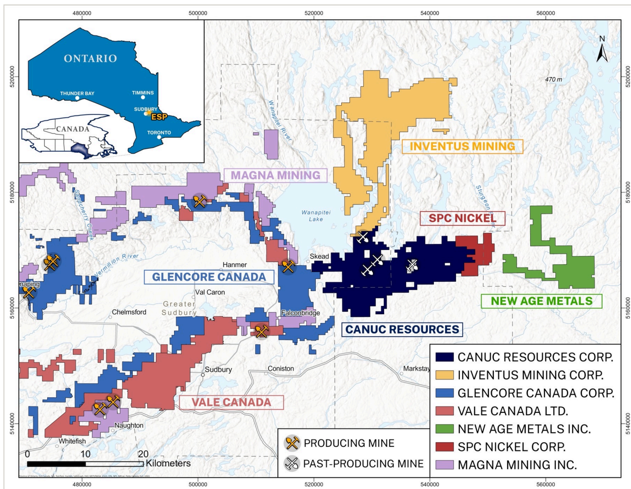
Figure 1. Canuc's East Sudbury Project (ESP) Regional Setting
